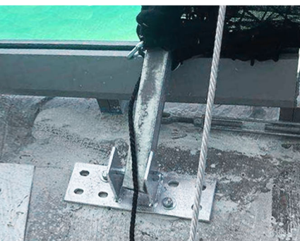
Bolt-On-Bracket
