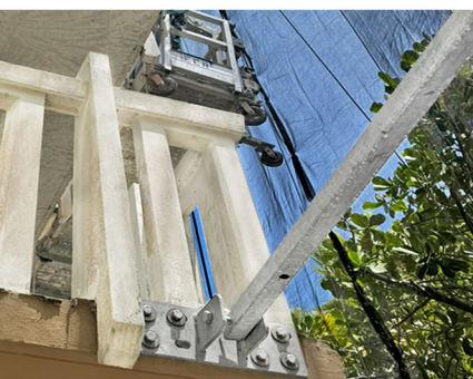
Bolt-On-Bracket
